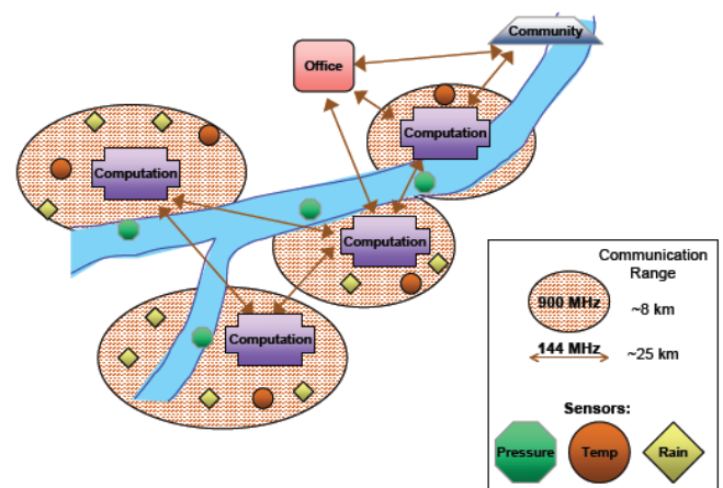
Fig -1: Flood Alert System Model [2]
