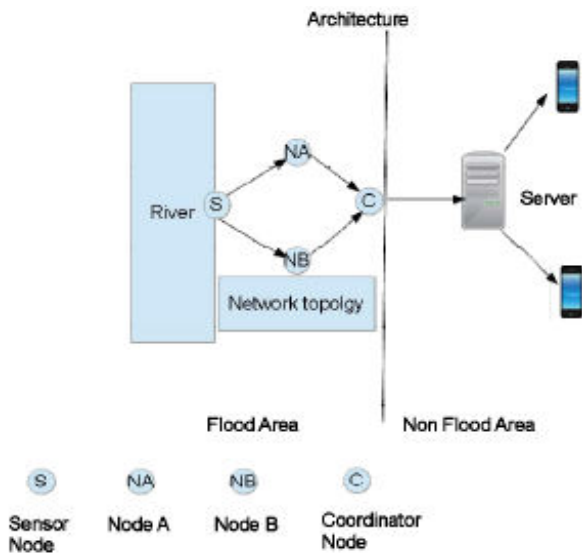
Fig -2: Flood Flood Alert System Model [5]
